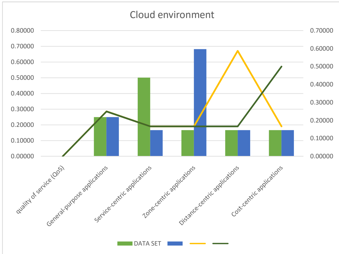
Figure 1. Cloud environment
