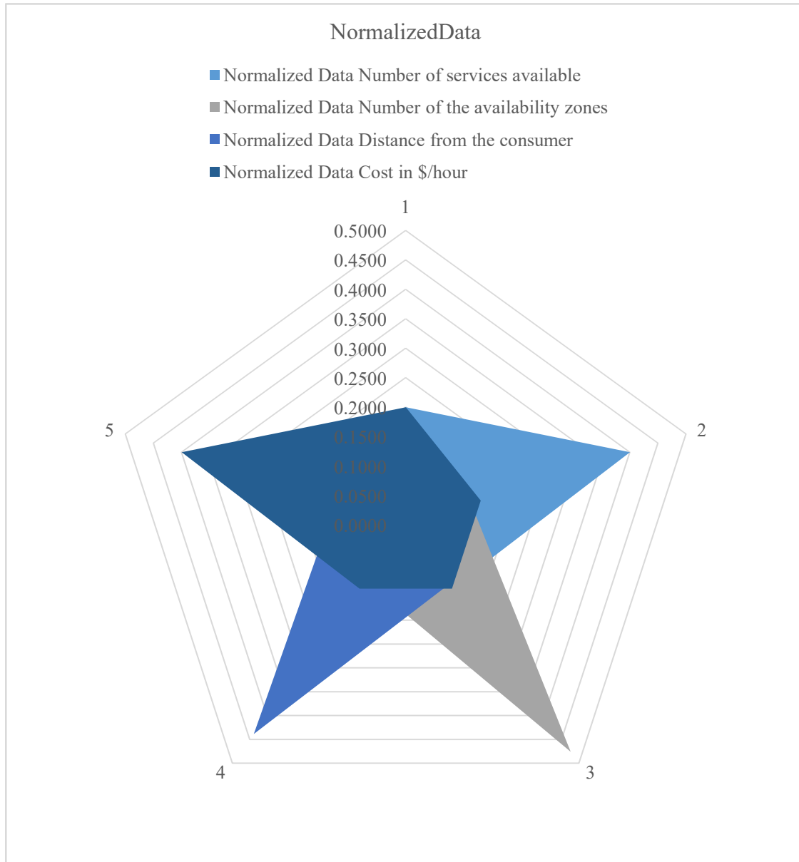
Figure 2. Normalized Data
