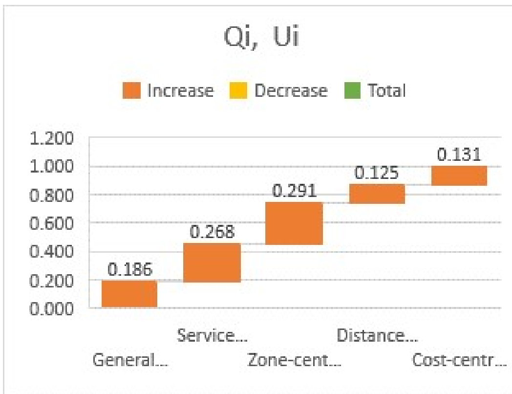
Figure 4. Q_i , U_i
